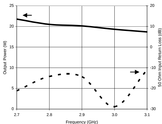
ILT2731M15 : Pin = 2W / 100us / 10% / 28V / Idq=10mA
